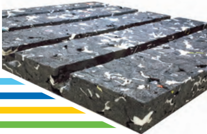
Machined Drain Channels
